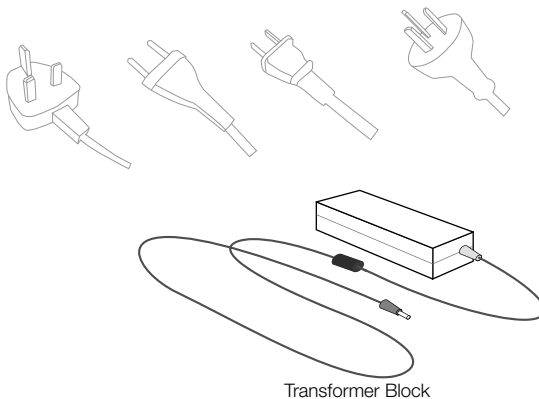
Transformer Block
